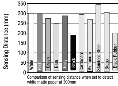
Color (100×100mm matte paper), material vs. Sensing Distance (Preset 300mm)
