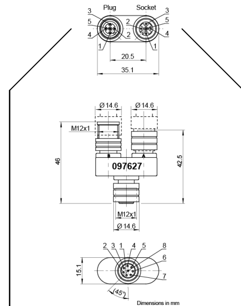
Y-distributor HS9Z-H3YD
