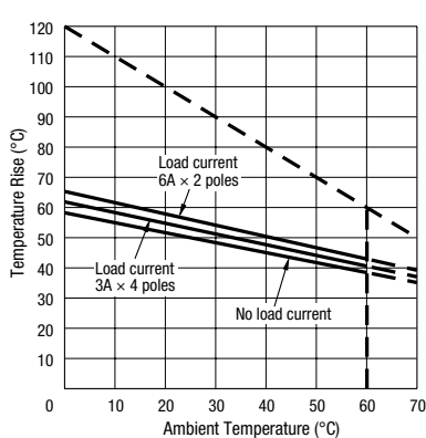
RU4/RU42 (AC Coil, 50 Hz)
